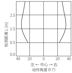
• BJR3M-PDT-F
