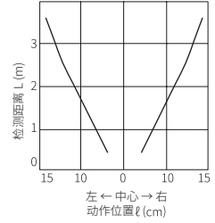
• BJR3M-PDT-F
