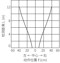
• BJR10M-TDT-F
